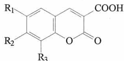
3-carboxycoumarines
