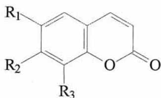
Coumarines
