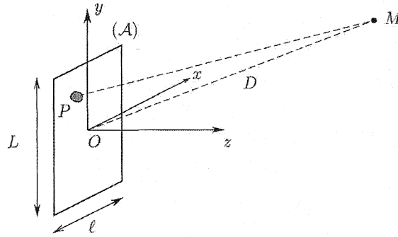
FIGURE 1 – Antenne rectangulaire
