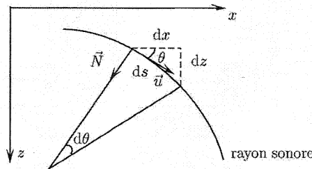
FIGURE 10 – Rayon sonore
